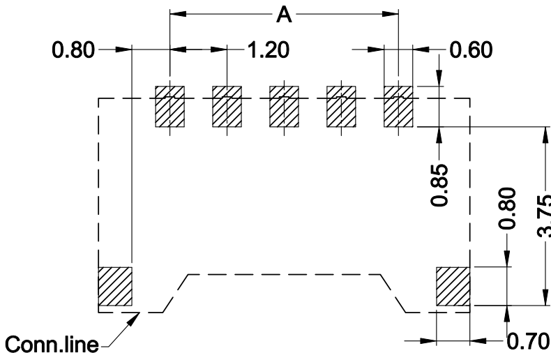
Recommended P.C.B Layout General Tolerance±0.05
